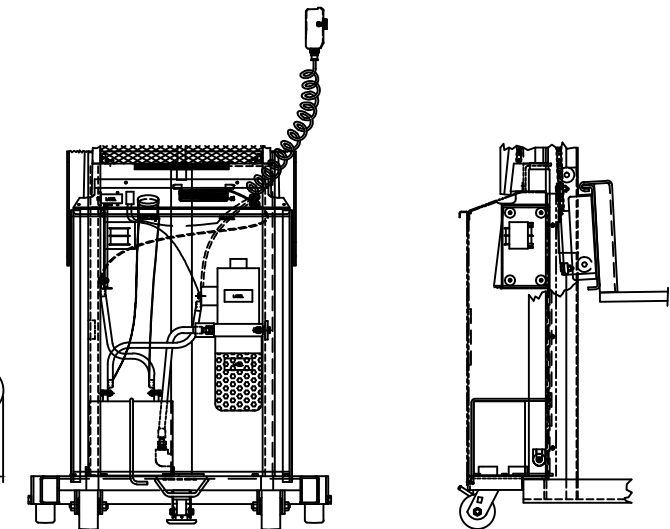
POWER UNIT
