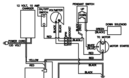
WIRING DIAGRAM
