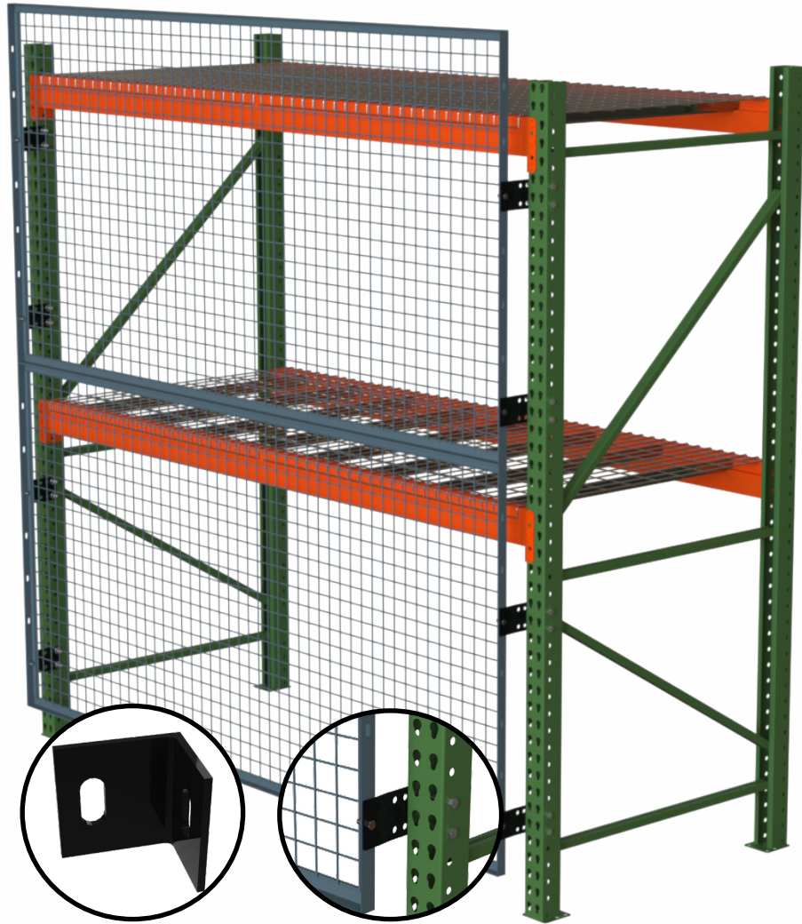
Offset brackets are available in 1" - 3" and 4" - 6".
